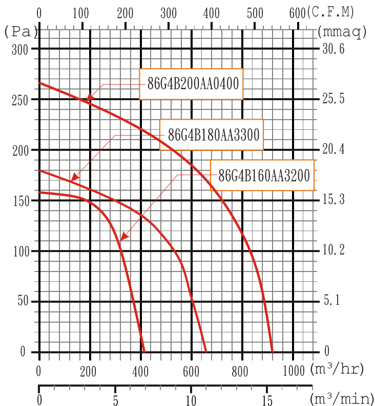
50Hz-4Pole
