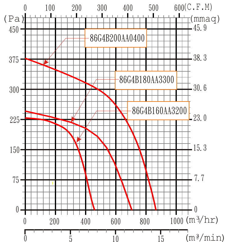
60Hz-4Pole
