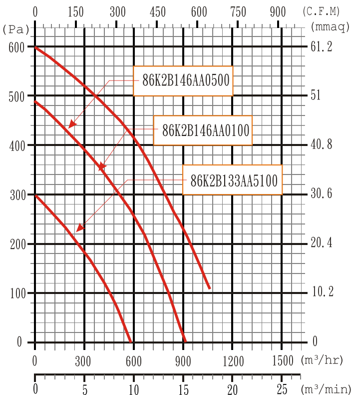
60Hz-2Pole
