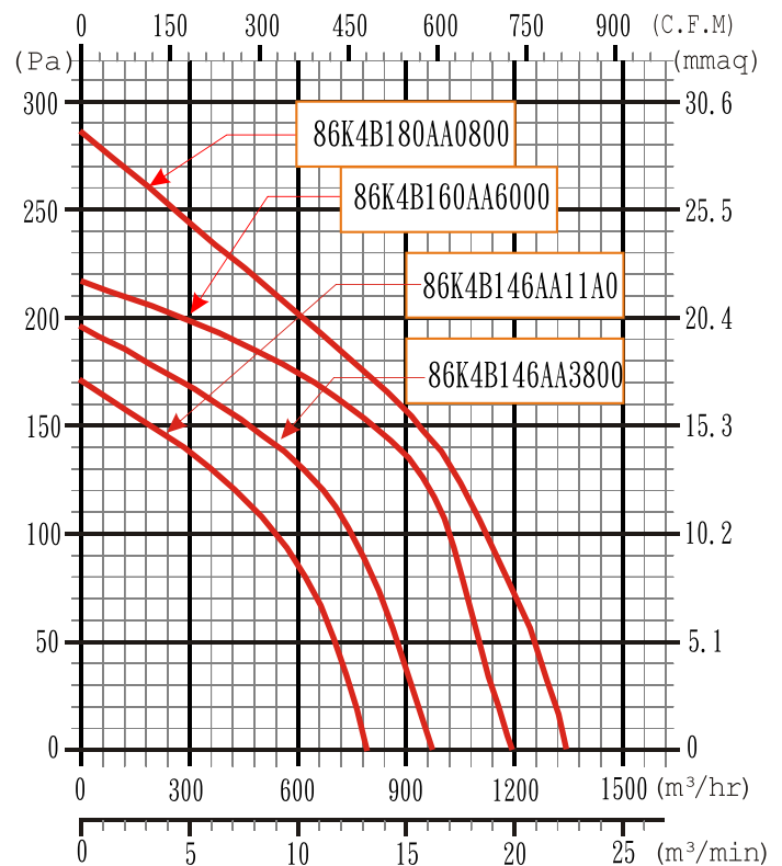
60Hz-4Pole
