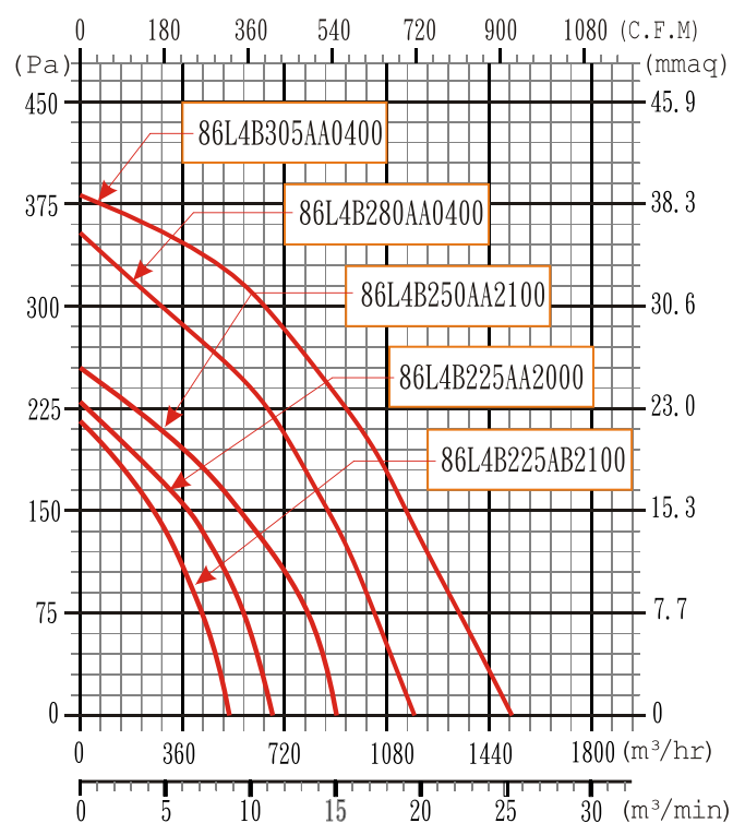
60Hz-4Pole
