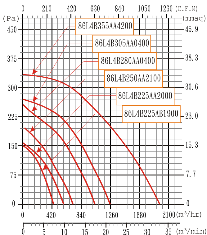
50Hz-4Pole
